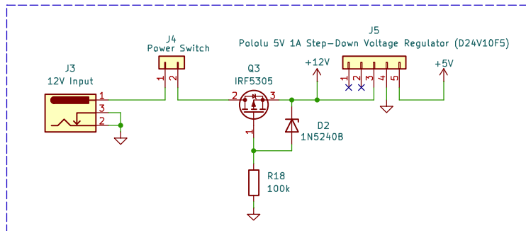
Option 1: 12V via barrel jack and 5V only using onboard regulator:
