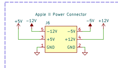
Option 2: Apple II compatible connector for providing all 4 voltages:
